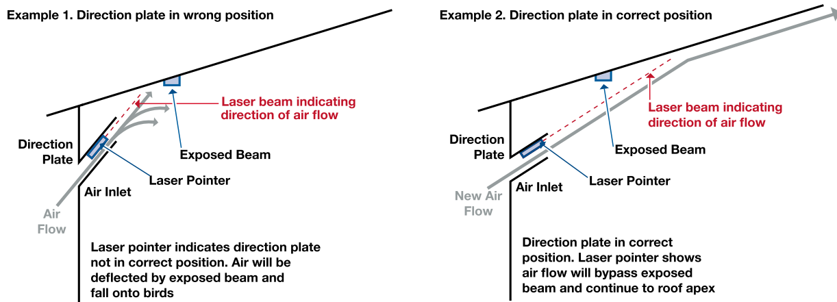
Figure 6.8: Using a laser pointer to provide a visual reference of direction of airflow into the house to determine if the air direction plate is positioned correctly. The direction plate can then be set to ensure that airflow bypasses any ceiling obstructions.
